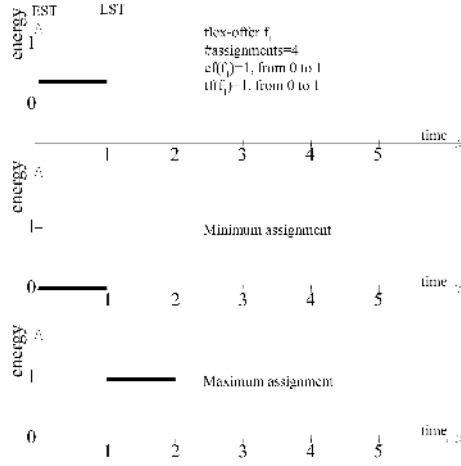
Fig. 2.2: Time series definition example with ef(f_1) = 1 and lf(f_1) = 1
