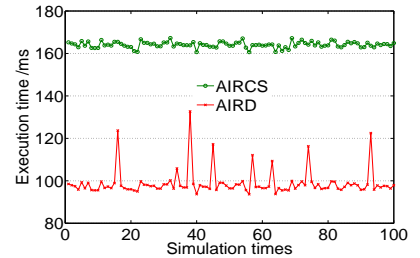
Fig. 3. Execution time.
