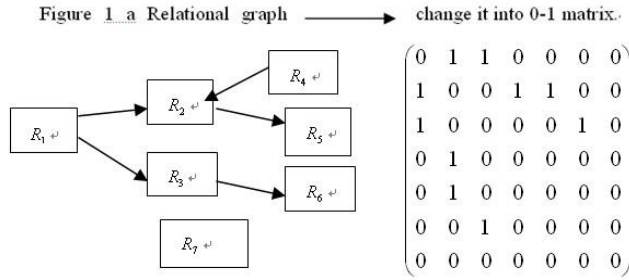
Figure 2 the result of Figure 1 into 0-1 matrix
