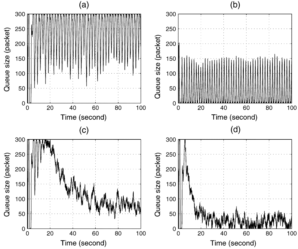
Fig. 7. System responses for DropTail, RED, PI, and REM.
