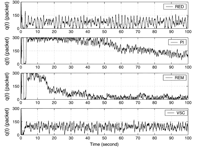
Fig. 13. Performance in the presence of short-lived TCP flows.
