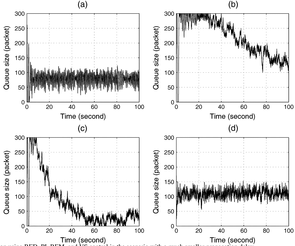
Fig. 14. Queue evolution using RED, PI, REM, and VS control in the scenario with a much smaller propagation delay.
