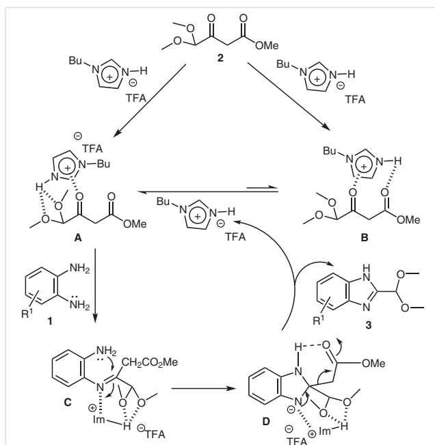
Scheme 3 Plausible mechanism for dual activation of 2 by [HBIm]TFA and catalytic cycle in the synthesis of acetal 3
