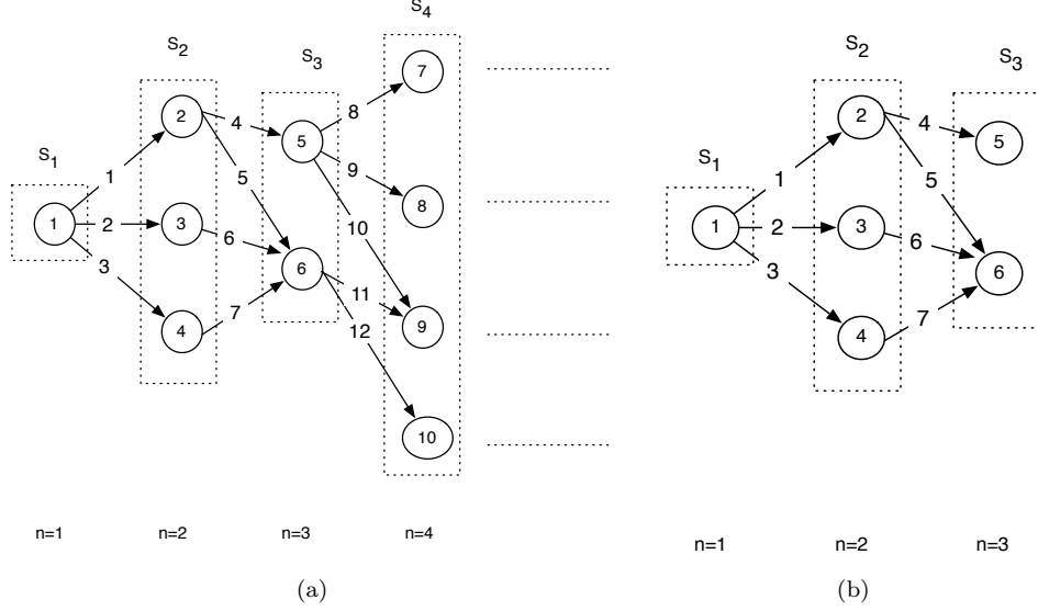
Figure 3: (a) An illustration of a non-stationary infinite-horizon discounted deterministic dynamic programming network. (b) A two-horizon truncation of the network in (a). States numbered 5 and 6 are “terminal”.
