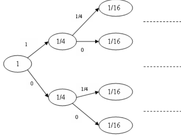
Figure 1: An infinite network flow problem.
