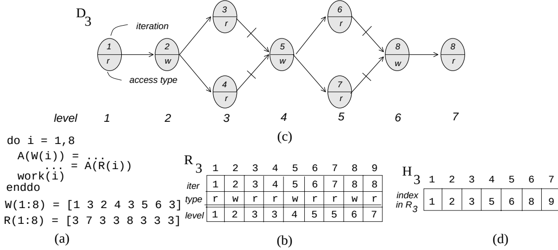
Figure 2: A (a) source loop, (b) the array R_3 for A[3] , (c) its dependence graph D_3 , and (d) its hierarchy vector H_3 .
