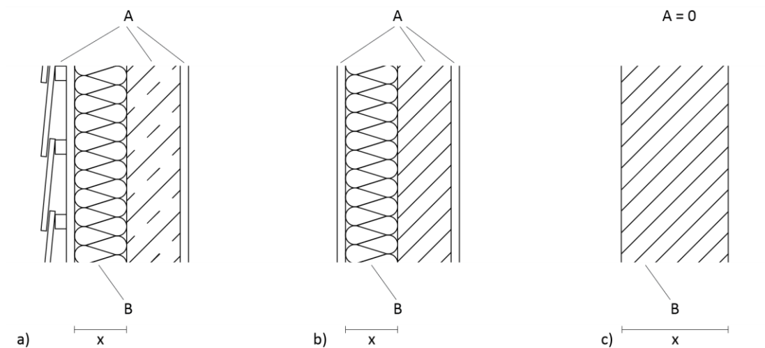
Figure 26: Examples for simplified component input: a) ventilated façade with wooden cladding and reinforced concrete wall, b) External Thermal Insulation Composite System (ETICS) on lime sand stone, c) monolithic light weight concrete
