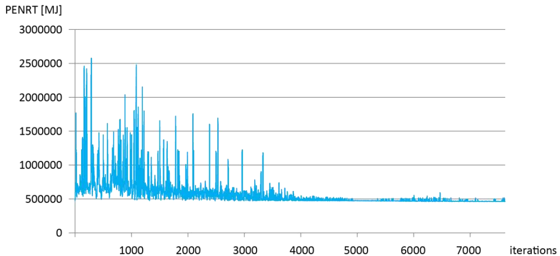
Figure 40: Best combination of insulation material and thickness for PENRT_{LC} and HP 4.8 mix and process of optimization
