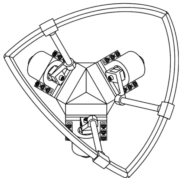
Fig. 2. Physical model of spherical DT.
