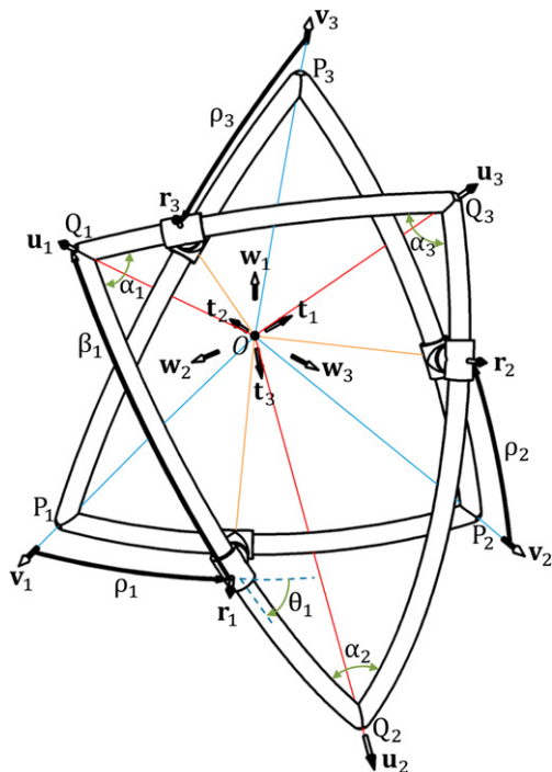
Fig. 1. General model of spherical DT.
