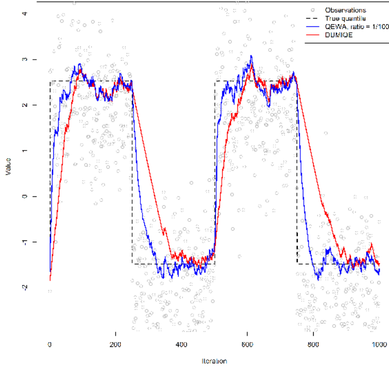
Fig. 1 Quantile estimates in every iteration using the DUMIQE and the suggested algorithm QEWA using ratio \gamma/\lambda = 1/100 .
