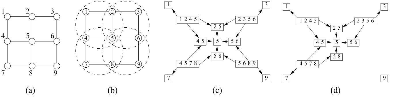
Fig. 15. Kikuchi clustering on the grid. (a) Original two-dimensional grid. (b) Clustering into groups of four. (c) Associated hypergraph with maximal hyperedges of size M = 4 . (d) One acyclic hypergraph of width three embedded within (c).
