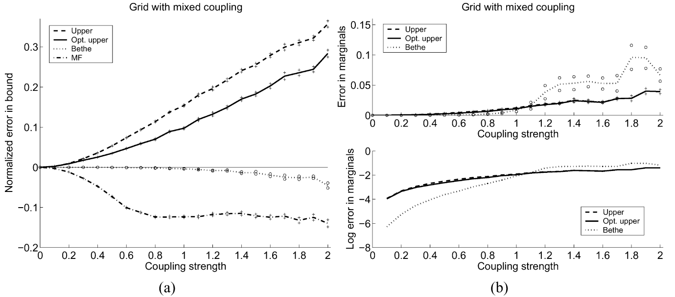
Fig. 8. Comparisons of convex upper bounds, mean field (MF), and the Bethe approximation for mixed couplings on a grid-structured model. (a) Comparison of the normalized error in the bounds (and Bethe approximation) to the log partition function. (b) Comparison of the error in the approximate marginals.
