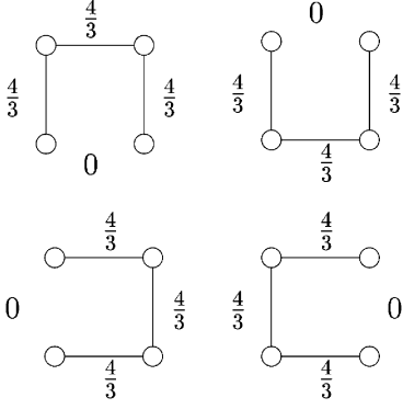
Fig. 4. A convex combination of four distributions p(\mathbf{x}; \theta(T_i)) , each defined by a spanning tree T_i , is used to approximate the target distribution p(\mathbf{x}; \bar{\theta}) on the single-cycle graph.
