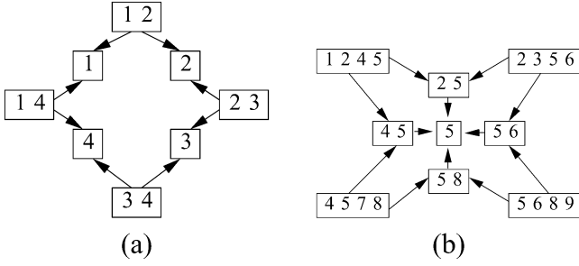
Fig. 12. Graphical representations of hypergraphs. Subsets of nodes corresponding to hyperedges are shown in rectangles, whereas the arrows represent inclusion relations among hyperedges. (a) An ordinary single-cycle graph represented as a hypergraph. (b) A more complex hypergraph that does not correspond to an ordinary graph.
