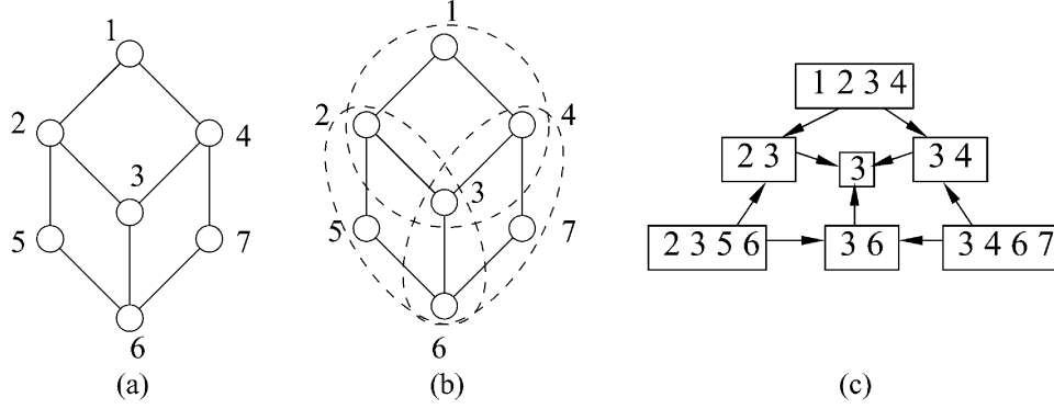
Fig. 13. Hypergraphs arise naturally by clustering operations. (a) Original pairwise MRF. (b) Particular clustering of the nodes. (c) Hypergraph defined by the clusters, as well as intersections between clusters, and intersections of intersections (node 3).
