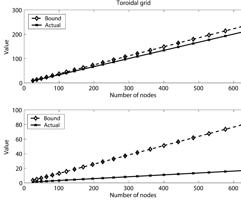
Fig. 11. Scaling of the bounds as a function of the number of nodes N in a four-nearest-neighbor grid with toroidal boundary conditions and homogeneous interactions between neighbors. (Top) Case of relatively weak coupling J = 0.2 in the spin representation of the Ising model. (Bottom) Case of stronger coupling ( J = 0.5 ).
