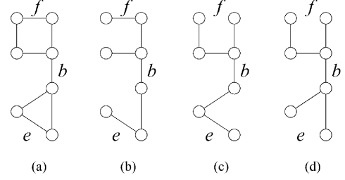
Fig. 3. Illustration of the spanning tree polytope \mathbb{T}(G) . Original graph is shown in panel (a). Probability 1/3 is assigned to each of the three spanning trees \{T_i \mid i = 1, 2, 3\} shown in panels (b)–(d). Edge b is a so-called bridge in G , meaning that it must appear in any spanning tree. Therefore, it has edge appearance probability \rho_b = 1 . Edges e and f appear in two and one of the spanning trees, respectively, which gives rise to edge appearance probabilities \rho_e = 2/3 and \rho_f = 1/3 .
