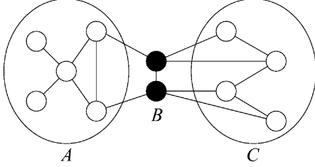
Fig. 2. Illustration of the relation between conditional independence and graph separation. Here the set of nodes B separates A and C , so that for a MRF, \mathbf{x}_{A|B} and \mathbf{x}_{C|B} must be conditionally independent.
