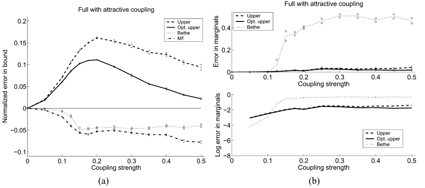
Fig. 9. Comparisons of convex upper bounds, mean field (MF), and the Bethe approximation for attractive couplings on a fully connected graph. (a) Comparison of the normalized error in the bounds (and Bethe approximation) to the log partition function. (b) Comparison of the error in the approximate marginals.
