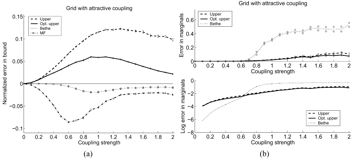
Fig. 7. Comparisons of convex upper bounds, mean field (MF), and the Bethe approximation for attractive couplings on a grid-structured model. (a) Comparison of the normalized error in the bounds (and Bethe approximation) to the log partition function. (b) Comparison of the error in the approximate marginals.
