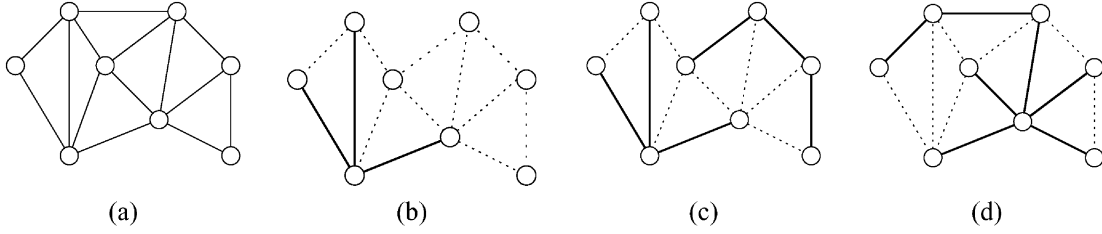
Fig. 1. (a) Graph with cycles. (b) A tree is a cycle-free subgraph. (c) A forest is a disjoint union of trees; it is spanning if it reaches every vertex of the graph. (d) A spanning tree reaches every vertex of the graph.
