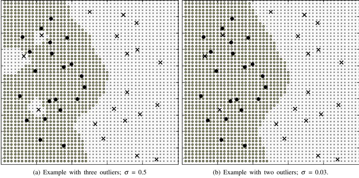
Figure 2: Example illustrating the implicit control of overfitting with \sigma .
