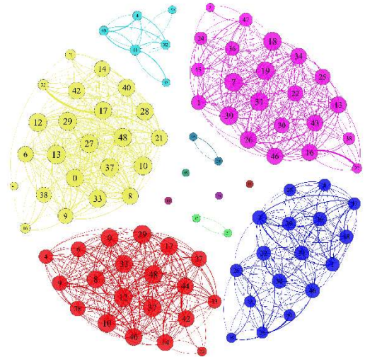
FIGURE 4. The basic temporal conflict network.
