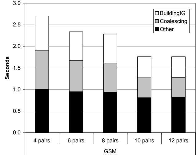
Figure 7. Register-allocation times for the GSM benchmark, as compiled for an imaginary Alpha family with floating-point register pairs. The horizontal axis shows the number of single-precision register pairs comprising the floating-point register pool. The vertical axis shows the total number of seconds required for register allocation of the entire GSM benchmark.
