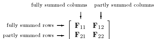
Figure 1: Partitioning of a frontal matrix.
