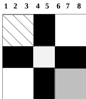
Figure 3: Supervariable detection for matrices in elemental format.
