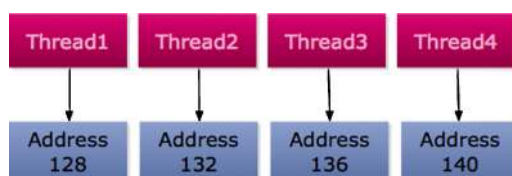
Figure 2. An example of coalesced memory access (by Johan Seland).
