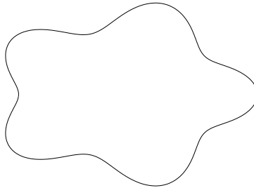
FIGURE 5.1. The contour \Gamma used in (5.1).
