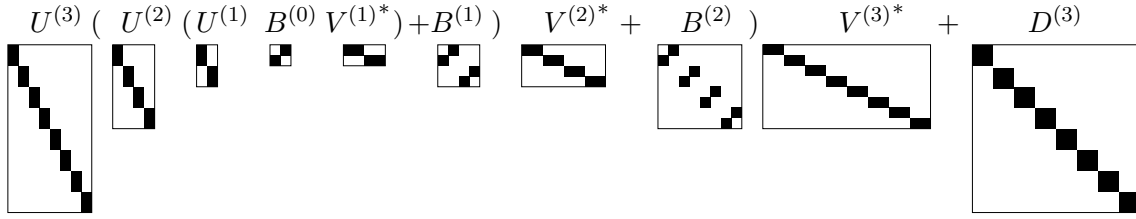
FIGURE 3.4. Block structure of formula (3.10).
