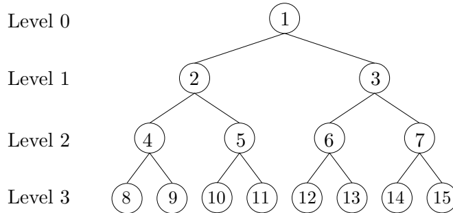
FIGURE 3.2. Numbering of nodes in a fully populated binary tree with L = 3 levels.
