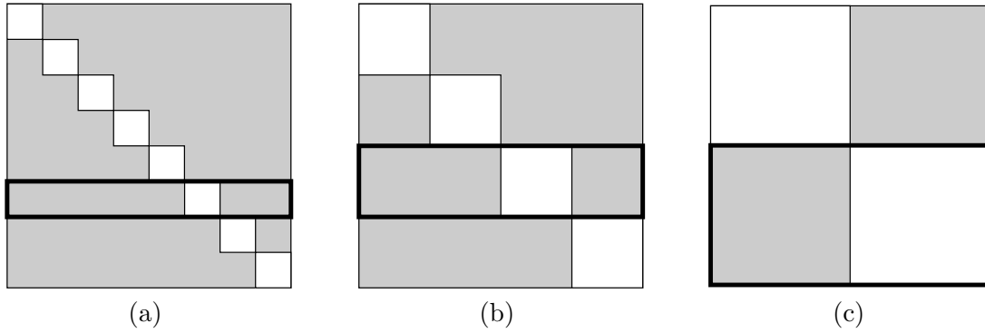
FIGURE 3.3. (a) The matrix A - D^{(3)} with non-zero parts shaded. The HSS row block A_{13}^{\text{row}} is marked with a thick border. (b) The matrix A - D^{(2)} with A_6^{\text{row}} marked. (c) The matrix A - D^{(1)} with A_3^{\text{row}} marked.
