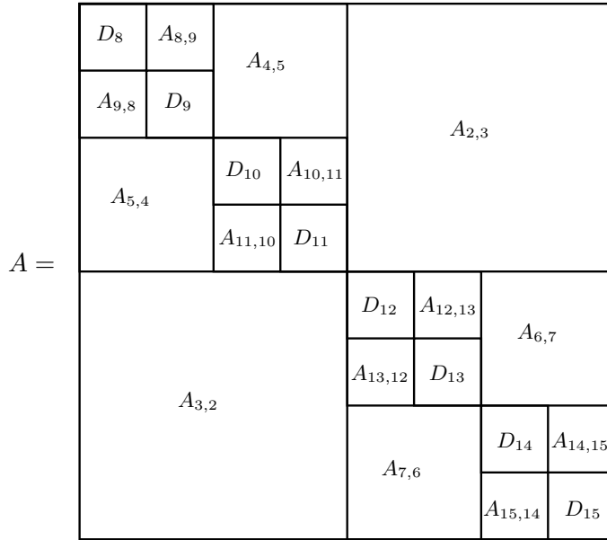
FIGURE 3.1. A matrix A tessellated in accordance with the tree in Figure 3.2.
