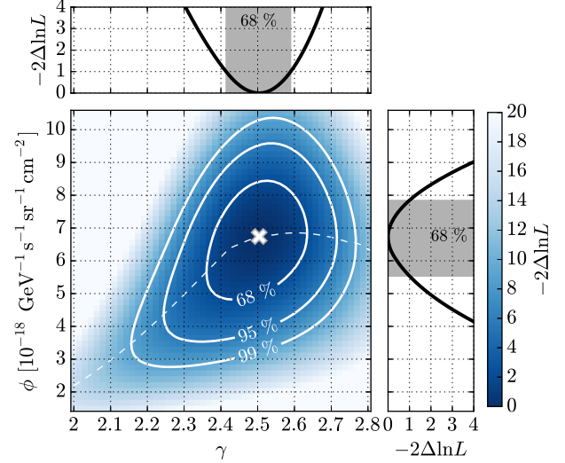
Figure 1. Profile likelihood scans around the best fit of the single power law model. The large panel displays a two-dimensional scan of the normalization \phi and the spectral index \gamma of the astrophysical neutrino flux; one-dimensional scans are shown in the small panels. The best-fit point is marked with “x” in the large panel, the dashed line shows the conditional best-fit value of \phi for each value of \gamma .
