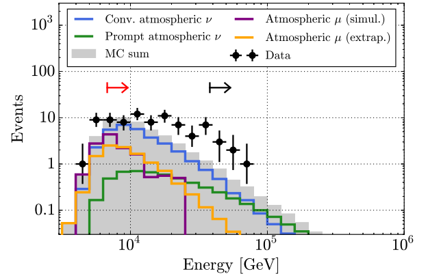
Figure 10. Same as Figure 9, but at final selection level. Additionally, an extrapolation of the muon background is shown in yellow. The gray filled histogram shows the sum of the two atmospheric neutrino components and the extrapolated muon background. The original work used events above 38 TeV (black arrow), here we use the data above 7 TeV (red arrow).
