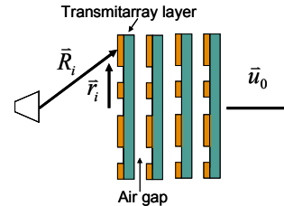
Figure 1. Transmitarray geometry
