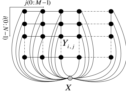
Figure 2. The graphical structure of 2D CRFs
