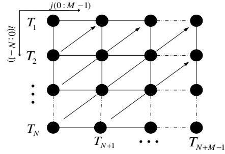
Figure 3. The diagonal state sequences of a 2D grid
